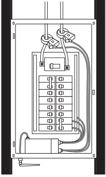
Flush Mounted (Interior)
