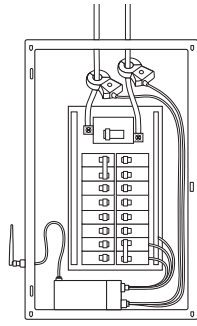
Surface Mounted (interior)
